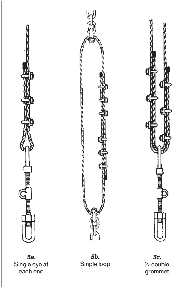
Fig 5. Configurations tested
